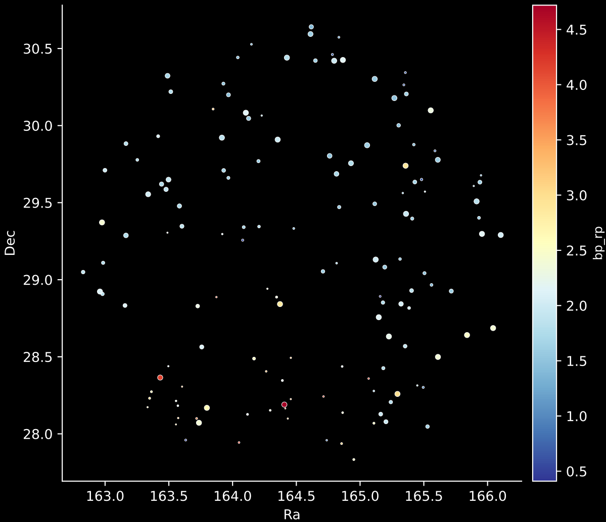
APOGEE DR17 Field: [TAUL1495_btx] Stars: 143
