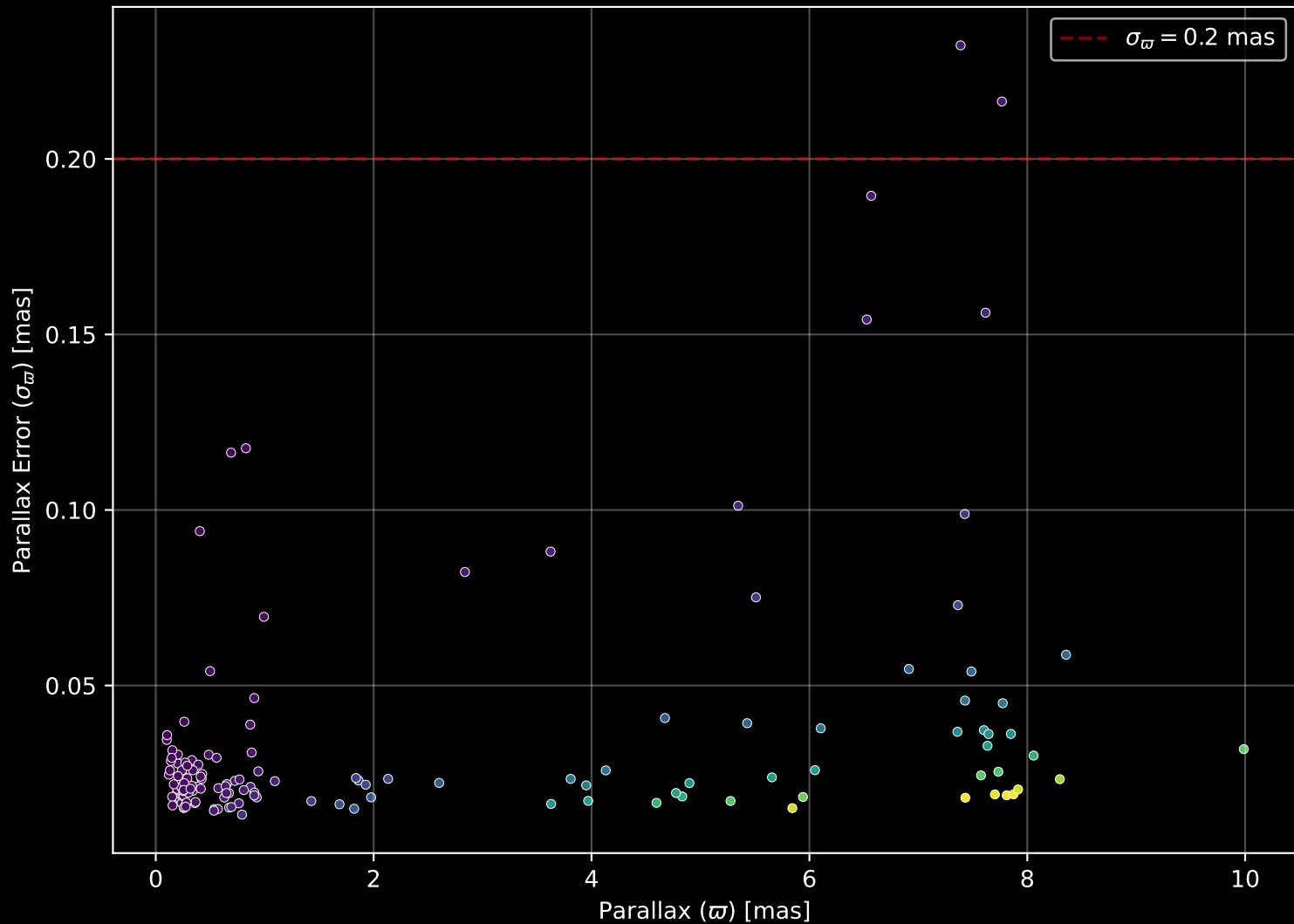
APOGEE DR17 Field: [TAUL1495_btx] Parallax Quality (n= 143)
