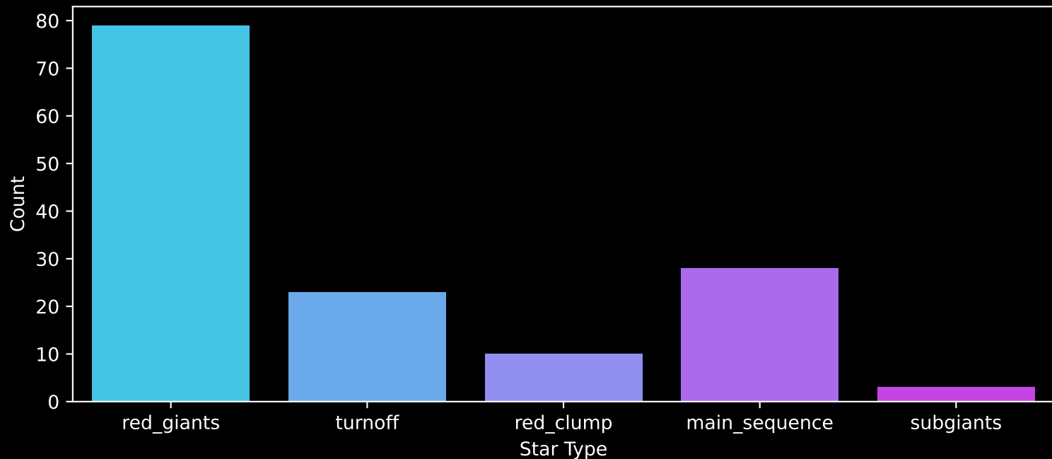
APOGEE DR17 Field: [TAUL1495_btx] Count plot of Star Type
