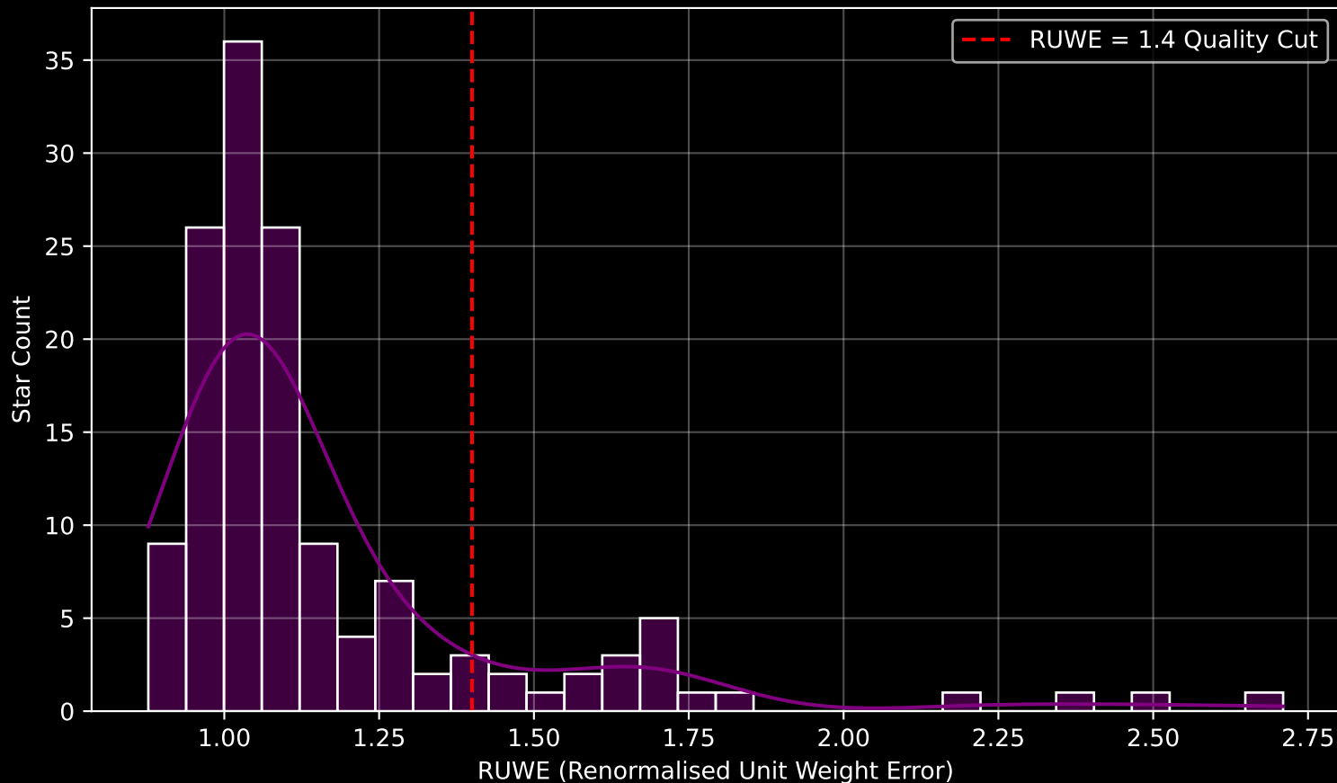
GAPOGEE DR17 Field [TAUL1495_btx] RUWE Distribution (n= 141)
