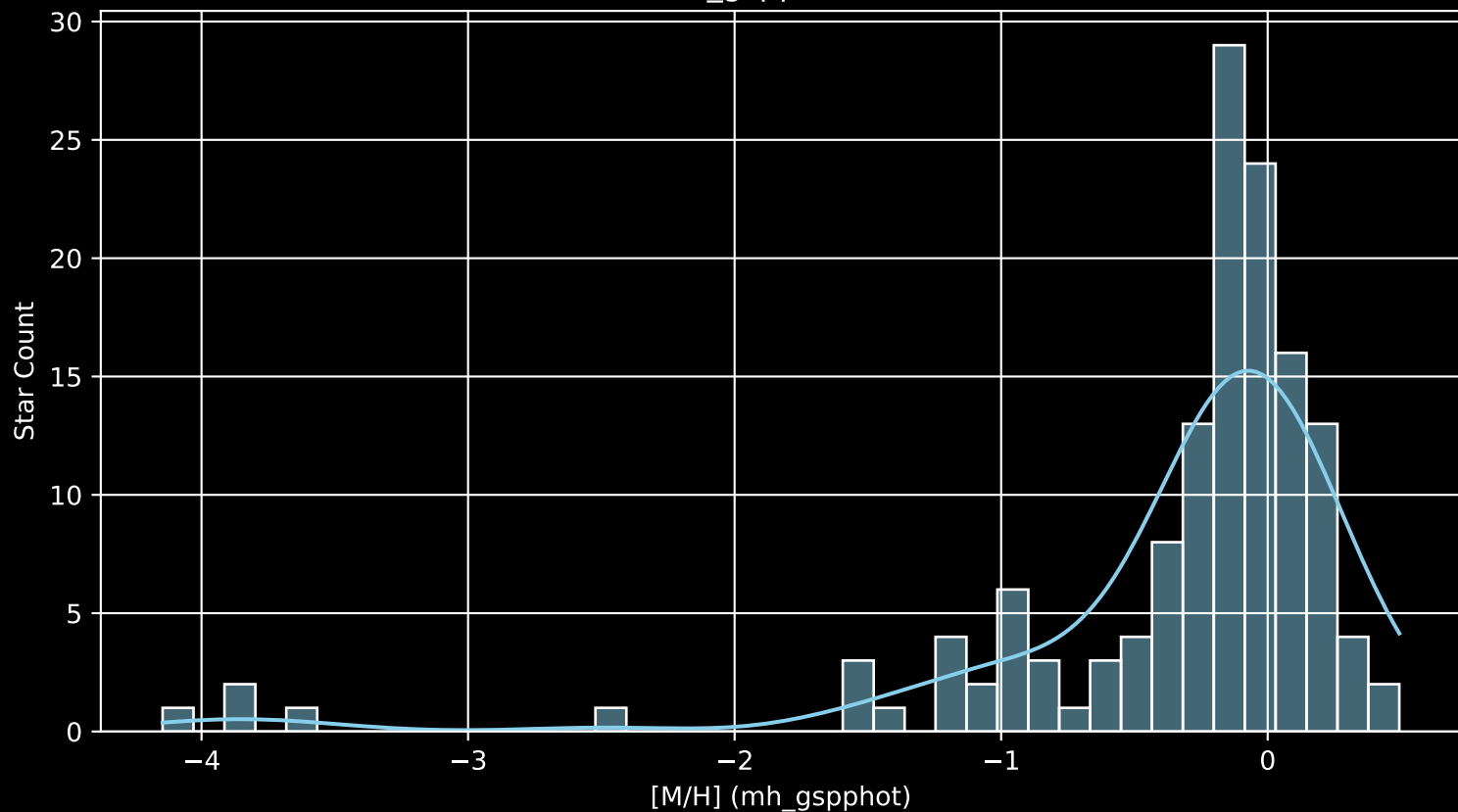
APOGEE DR17 Field: [TAUL1495_btx [M/H] (mh_gspphot) (n= 141)
