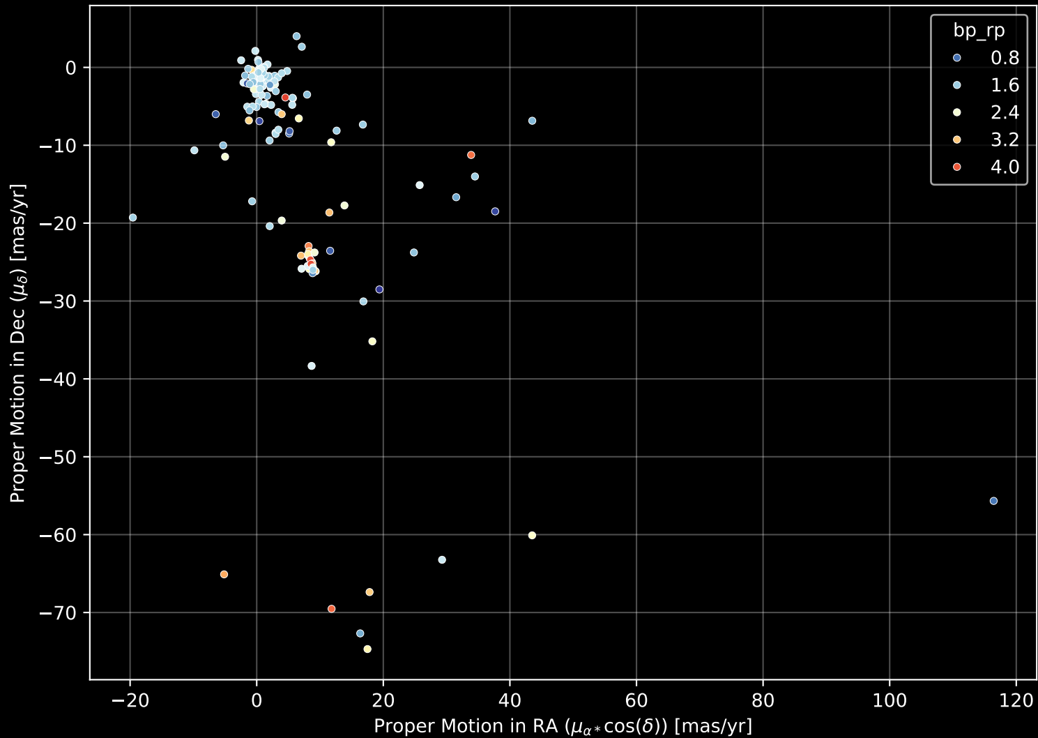
APOGEE DR17 Field: [TAUL1495_btx] Proper Motion Diagram (n= 143)
